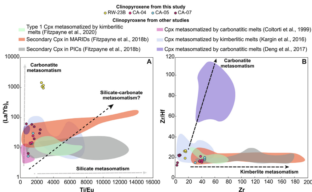
Fig. 8. Plots of La/Yb (PM-normalized) versus Ti/Eu (A), and Zr/Hf versus Zr (B) of studied clinopyroxenes from Carolina kimberlite mantle xenoliths. For comparison, were plotted clinopyroxenes formed by carbonatitic metasomatism (Coltorti et al., 1999; Deng et al., 2017); secondary clinopyroxenes found in MARIDs and PICs formed by kimberlitic metasomatism (Fitzpayne et al., 2018b, 2020), and clinopyroxenes of peridotites that were affected by kimberlitic or proto-kimberlitic metasomatism (Kargin et al., 2016; Fitzpayne et al., 2020).
