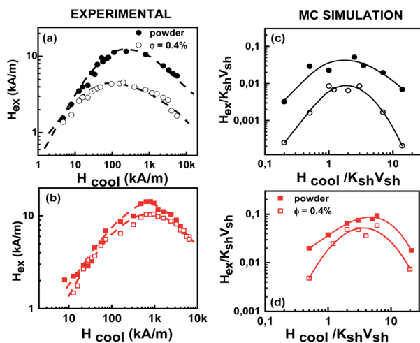
Fig. 2 Cooling field dependence of the exchange bias field H_{\text{ex}} extracted from hysteresis loops. Experimental data on the left panel (a and b) are compared with the Monte Carlo simulation results on the right panel (c and d) for frozen ferrofluid (open symbols) and a powder (full symbols) for the \text{MnFe}_2\text{O}_4/\gamma\text{-Fe}_2\text{O}_3 (a and c) and \text{CoFe}_2\text{O}_4/\gamma\text{-Fe}_2\text{O}_3 (b and d) core/shell nanoparticles respectively. The dashed and solid lines are guides to the eye.
