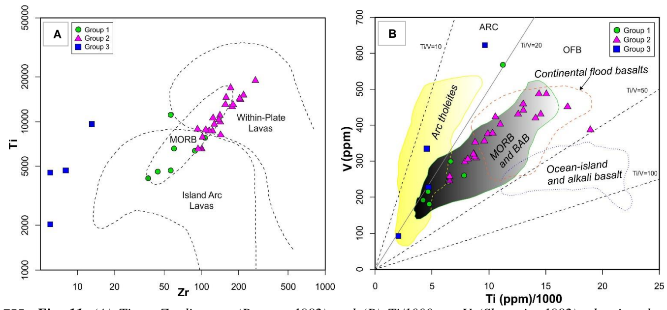
755 Fig. 11. (A) Ti vs. Zr diagram (Pearce, 1982) and (B) Ti/1000 vs. V (Shervais, 1982), showing the 756 fractionation trends observed in the metamafic rocks of the Rio Branco Suite (ARC-arc; MORB-mid-ocean 757 ridge basalt; BAB-back-arc basalt; OFB-ocean floor basalt).
