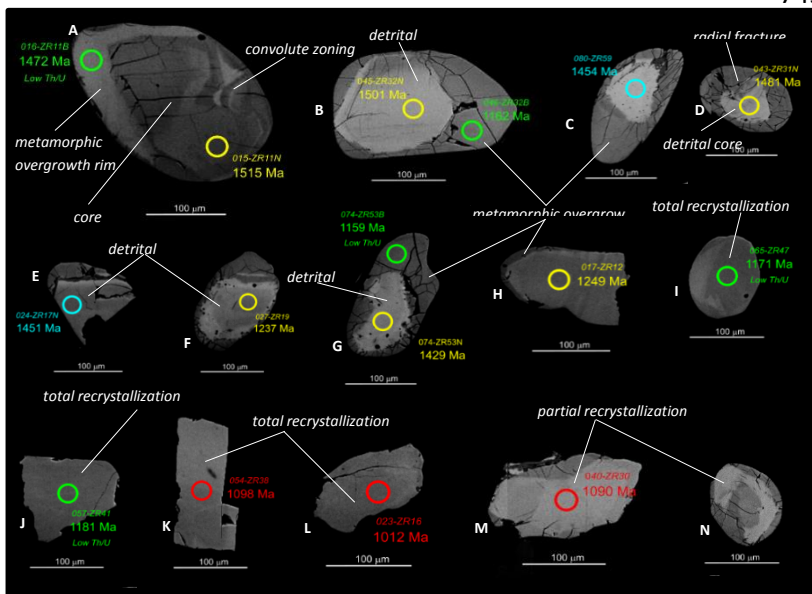
Fig. 9. BSE (Backscattered Electron) images of selected zircon grains of sample MQ-44 (calc-silicate gneiss of the Rio Branco Formation) showing usually recrystallized forms and varied internal morphologies. (A) zircon presenting core with high Th/U ratio, convolute zoning and overgrowth with low Th/U ratio (metamorphic rim). (B), (C), (D), (E), (F), (G) and (H) homogeneous and partially recrystallized zircon grains showing detrital core and metamorphic rims with low Th/U ratio and radial fractures. (I) sub-rounded and homogeneous zircon with low Th/U ratio. (J) homogeneous zircon fragment with
