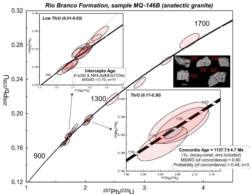
852 Fig. 15. U-Pb (LA-ICP-MS) Discordia and Concordia diagrams showing zircon 853 ages of the two main populations of anatectic granite (sample MQ-146B) in 854 paragneiss of the Rio Branco Formation. The age range of 1150-1136 Ma (n=3) 855 includes metamorphic and magmatic zircon grains based on BSE images and Th/U 856 ratios and provides an age of 1137.7 \pm 4.7 Ma. The range of 1021-986 Ma (n=11) 857 includes zircon grains with low Th/U ratio (0.01-0.03), rendering an intercept age 858 of 1011.3 \pm 9.6 Ma on the Discordia diagram.
