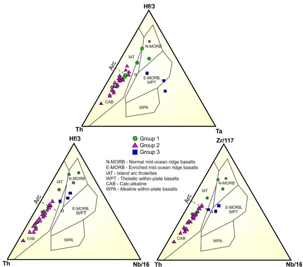
Fig. 13. Triangular diagrams of the Th-Hf-Ta-Zr-Nb system (Wood, 1980) used to identify the subduction components of the metamafic rocks from the Rio Branco Suite.
