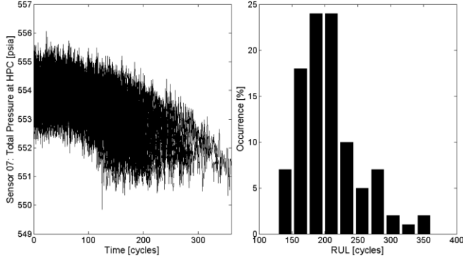
Figure 4. Sensor measurement and RUL distribution
