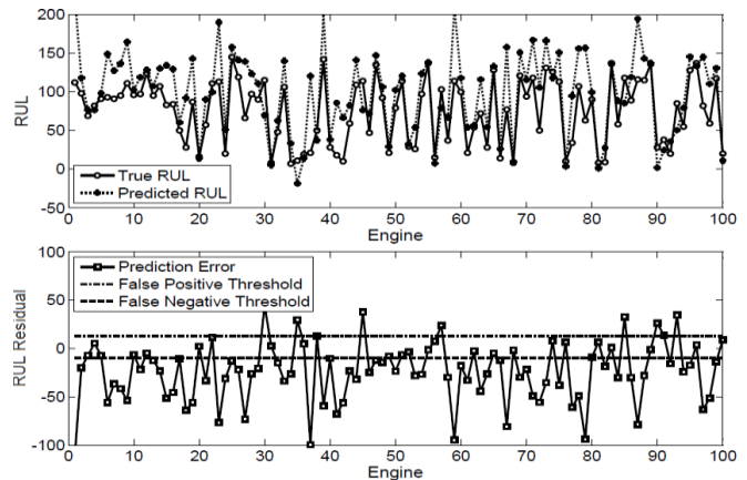
Figure 5. Classical ESN trained
