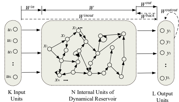
Figure 1. Basic Structure of ESN
