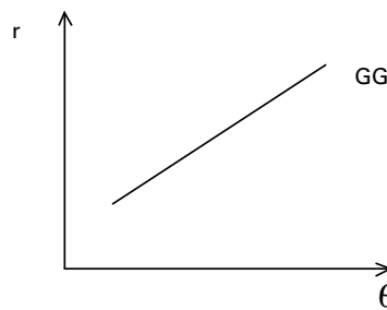
Figure 10: Locus GG
