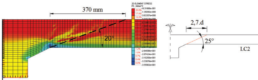
B Stress \sigma_{Max} on the rupture load of the slab model LC2 and the angle of the rupture surface experimental
