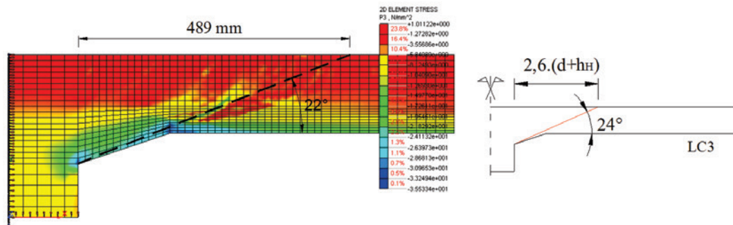
C Stress \sigma_{Max} on the rupture load of the slab model LC3 and the angle of the rupture surface experimental
