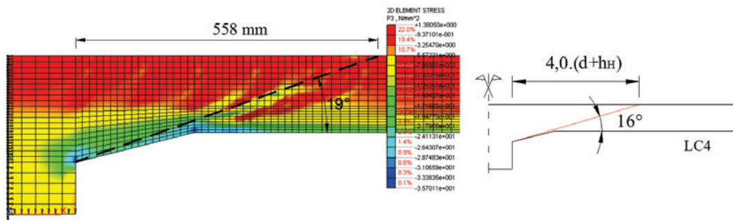
D Stress \sigma_{Max} on the rupture load of the slab model LC4 and the angle of the rupture surface experimental
