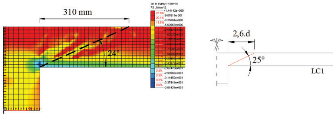
A Stress \sigma_{Max} on the rupture load of the slab model LC1 and the angle of the rupture surface experimental
