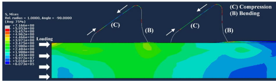
Figure 13 Deformed configuration and stress (Pa) distribution at the moment of ultimate load
