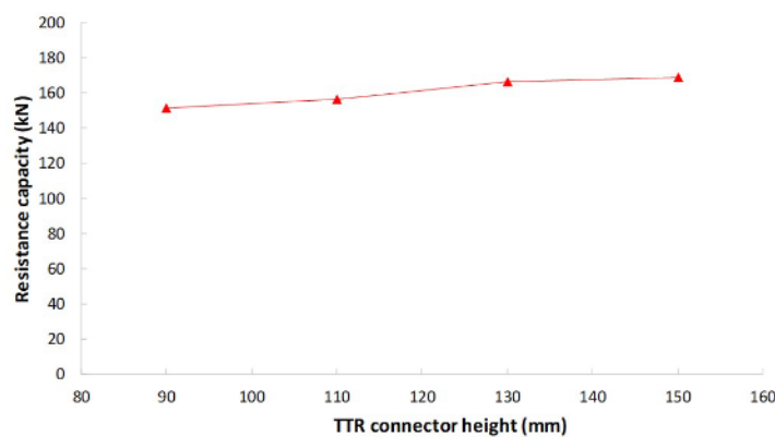
Figure 20 Resistance capacity for each height of the TTR connector
