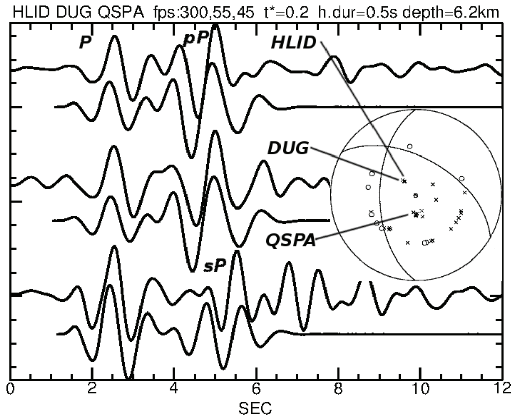
Figure 6 - Teleseismic P-wave modeling to determine the depth, with three stations (top to bottom): HLID, DUG (both in the United States) and QSPA (South Pole). The upper/lower traces are observed/calculated seismograms. Seismograms converted to WWSP response and modeled with a triangular source-time function with total duration 1.0 s and t^* = 0.2 . The pP phase appears 2.0 s after the P, with reversed polarity and sP phase appears 4.0 s after the P in QSPA station.
