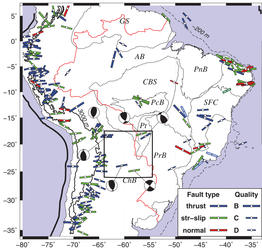
Figure 7 - Maximum horizontal stress direction from focal mechanism. The colors are the mechanism type and the size of bars (B, C and D) indicates the quality of the fault plane solution conform WSM – Project criteria (site: http://dc-app3-14.gfz-potsdam.de/index.html ). The bar direction corresponds to compressional axis (P-axis) in thrust and strike-slip and null axis (B-axis, the intersection of the two nodal planes) in normal faults. The rectangle shows the mechanisms used in the stress inversion in Fig. 8. The main geological provinces are the same as Fig. 1. Data from Assumpção et al. 2016.
