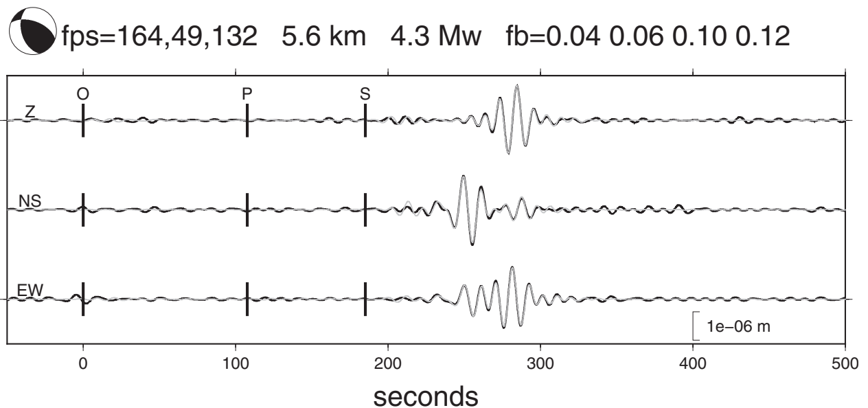
Figure 5 - Coxim event surface waves modeling using ISOLA program with CPSP methodology from Fojtíková and Zahradník (2014). In order, we have Z, NS and EW components in displacement (m) from BEB4B station (~ 800 km distance) with origin time (O), P and S-waves arrival marked. Observed data is the black line and synthetic is gray. The focal mechanism is shown in the top left with the depth, magnitude Mw and the frequency band used.
