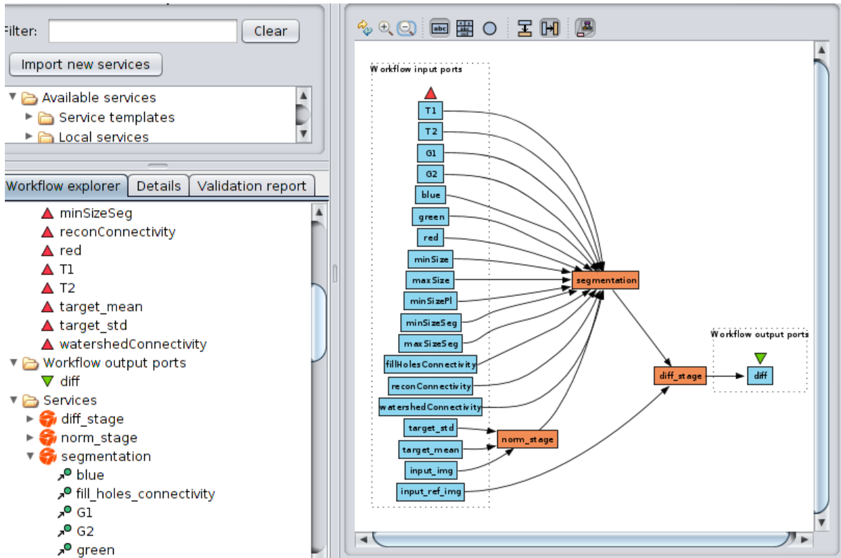
Figura 3.4: The example workflow described with the Taverna Workbench.
