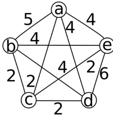
(b) Initial graph of instance example.
