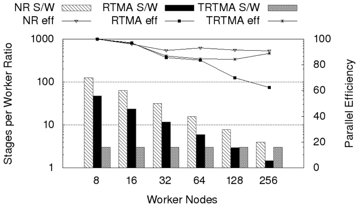
Figure 4.5: Combination of Stages per Worker Processes (S/W) and parallelism efficiency values. The S/W ratio for TRTMA was fixed as 3 for all WP values. The parallelism efficiency was calculated based on the previous execution (e.g. for WP 64, it is the execution time for WP 32 vs WP 64).
