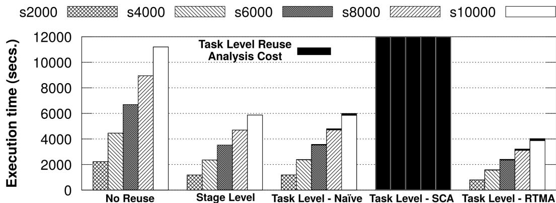
Figure 4.2: Impact of the computation reuse strategies for the VBD SA method.
