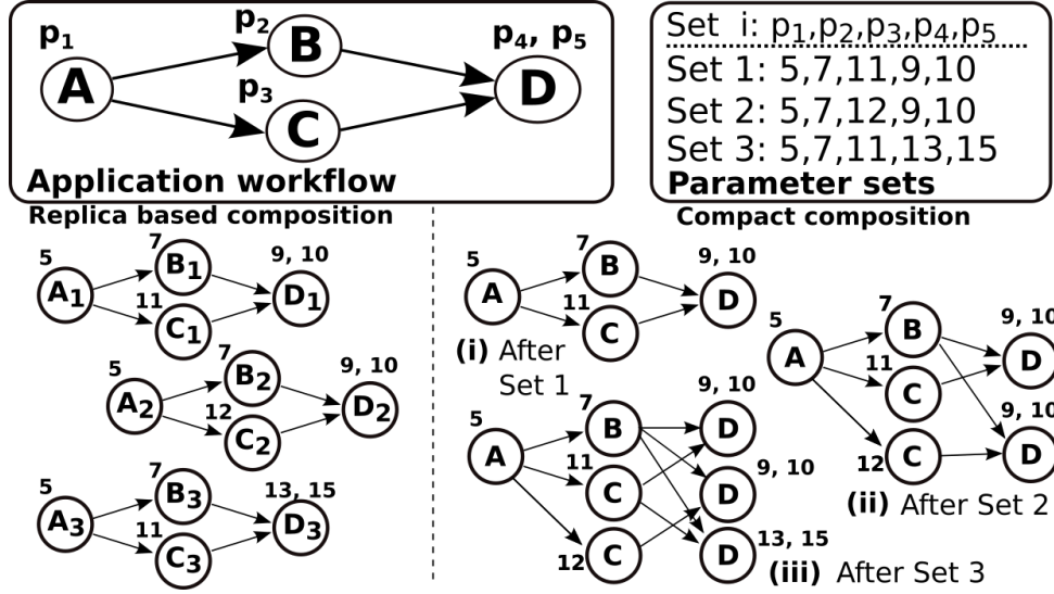
Figure 3.2: A comparison of a workflow generated with and without computation reuse. Image extracted from [42].
