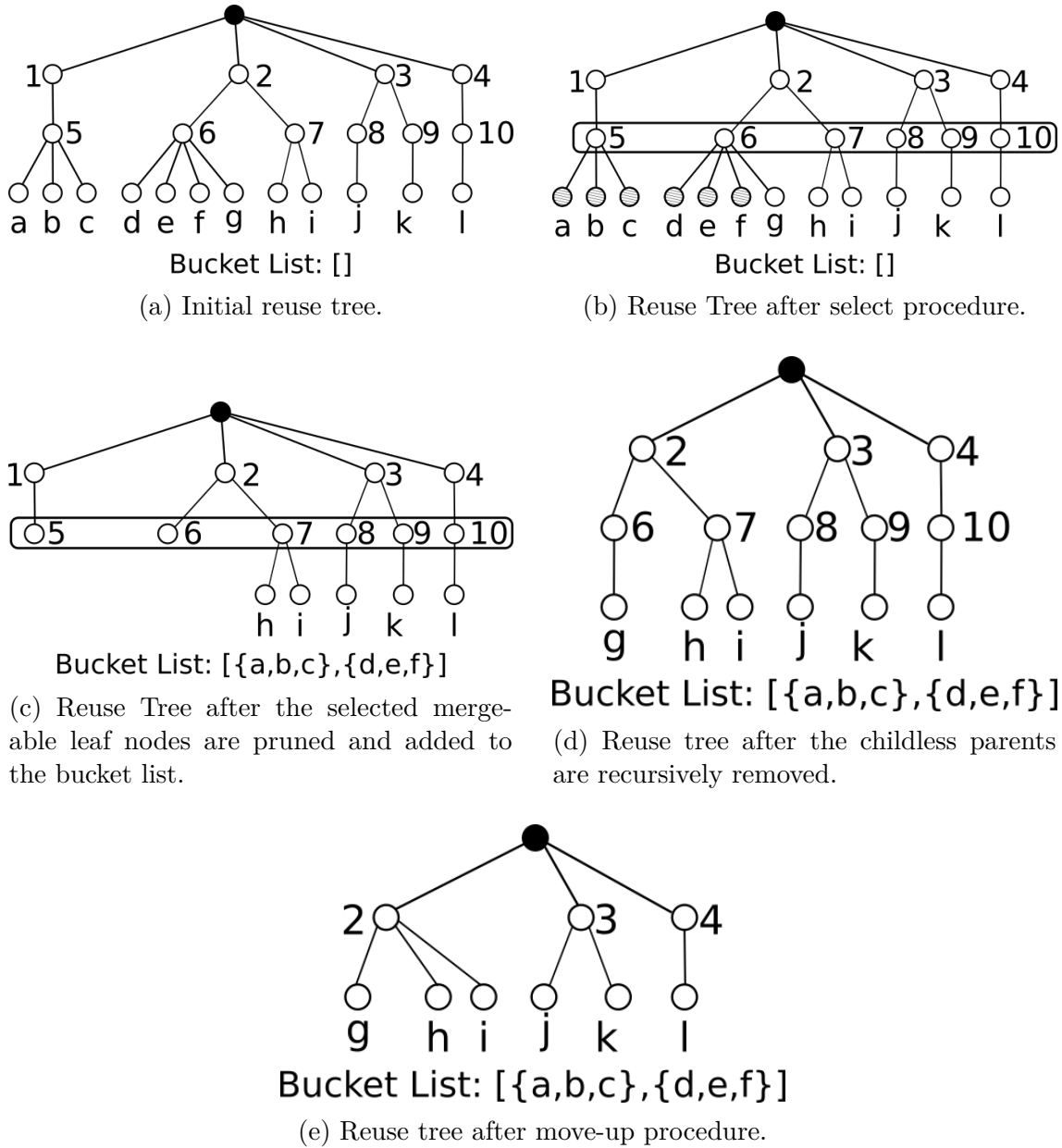
Figure 3.7: An example of Reuse Tree based merging with MaxBucketSize = 3 . The merged stages of each step are shown below the tree on the bucket list.
