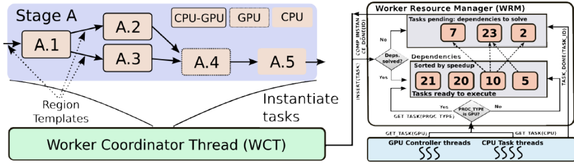
Figure 2.4: The execution of a stage instance from the perspective of a node, showing the fine-grain tasks scheduling. Image extracted from [39].
