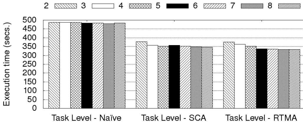
Figure 4.3: Impact of varying MaxBucketSize from 2 to 8.
