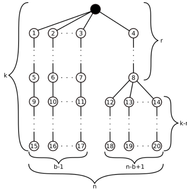
Figure 3.12: A general worst-case reuse-tree representation on which we have all n stages divided into b buckets. On this case we have b - 1 buckets with exactly one stage, and thus cost k . Hence, the last bucket has n - b + 1 stages. For this last bucket we assume the single and uniform reuse of the first r task, having no reuse for the remaining k - r tasks. This is the worst-case for balancing applications.
