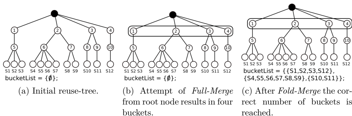
Figure 3.9: Another example of Full-Merge and Fold-Merge on which MaxBuckets is 3 and the exact division of stages cannot be reached by Full-Merge .
