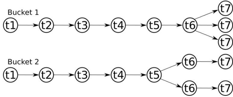
(a) Two example buckets and their reuse trees. Bucket 1 was the result of the merger of three stages, while Bucket 2 had two stages initially.
