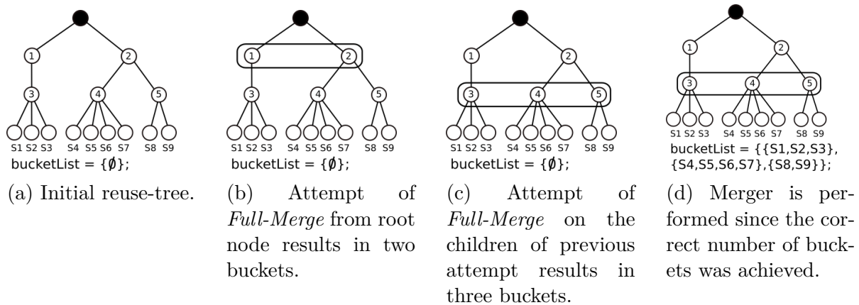
Figure 3.8: Simple example of Full-Merge on which MaxBuckets is 3 and the exact division of stages is reached.
