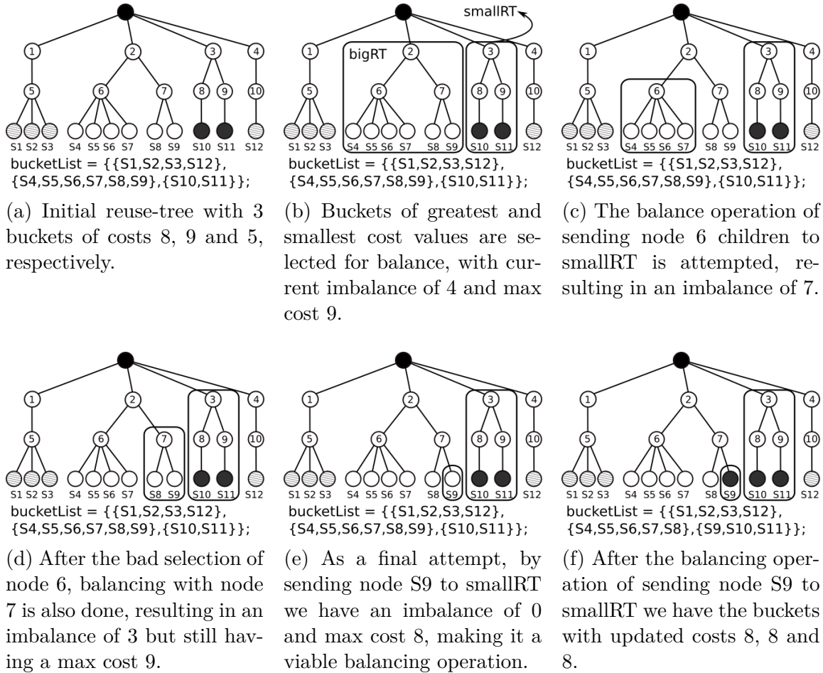
Figure 3.11: An example of the Balance step on which there are 3 buckets to be balanced.
