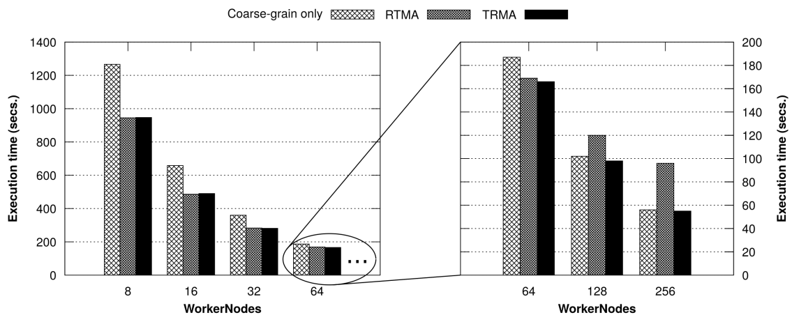
Figure 4.4: Comparison of the “no fine-grain reuse” (NR) approach with the RTMA and TRTMA. RTMA uses MaxBucketSize 10, while TRTMA uses MaxBuckets 3× the number Worker Processes (WP). The execution times for WP > 32 were zoomed in a separated figure for the purpose of better visualization.
