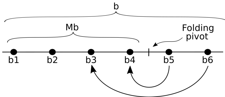
Figura 3.10: An example of a Fold-Merging of buckets b_1 - b_6 . Initially we start with b = 6 buckets, trying to achieve Mb = 4 buckets. In order to do so b - Mb merger operations are performed. The task cost of the buckets follows the ordering b_1 \geq b_2 \geq b_3 \geq b_4 \geq b_5 \geq b_6 .
