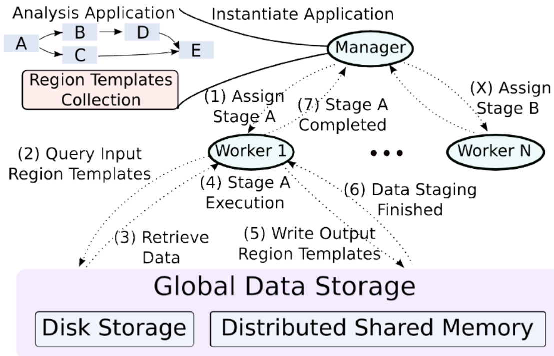
Figura 2.3: The main components of the Region Templates Framework, highlighting the steps of a coarse-grain stage instance execution. Image extracted from [39].
