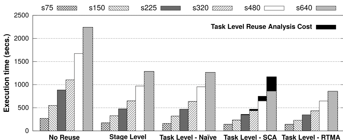
Figure 4.1: Impact of the computation reuse for different strategies as the sample size of the MOAT analysis is varied. E.g., s150 means that the experiment had 150 executions of the given workflow.
