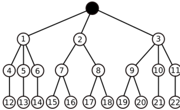
Figure 3.13: An example reuse-tree that can be used to illustrate possible prunable nodes. E.g., the use of nodes 4, 5, 6, or 10, 11 as an improvement attempt results in the same outcome (cost 3), making them interchangeable, as with nodes 7, 8 or 9 (cost 4), or nodes 12-22 (cost 3).
