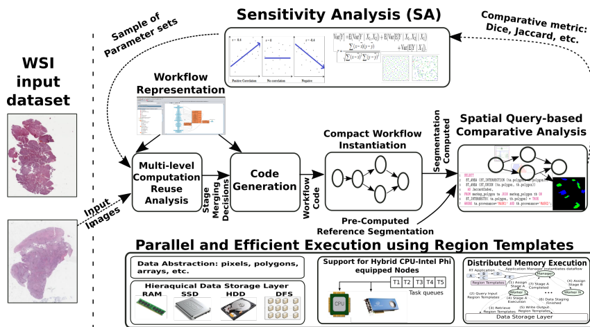
Figure 3.1: The parameter study framework. A SA method selects parameters of the analysis workflow, which is executed on a parallel machine. The workflow results are compared to a set of reference results to compute differences in the output. This process is repeated a set number of times (sample size) with varying input parameters' values.
