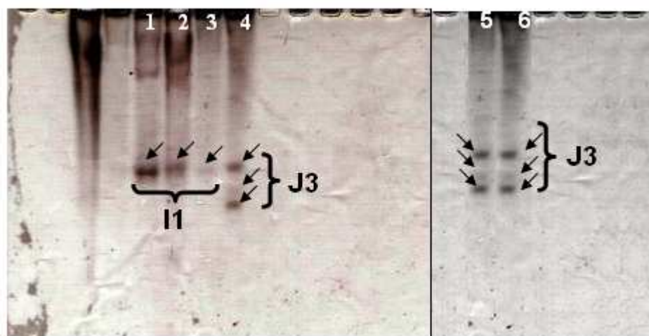
Figure 1 - Esterase phenotypes of M. incognita (I1) and M. javanica (J3) displayed in two polyacrylamide gels: Gel 1: Lonchocarpus muehlbergianus (1), Croton urucurana (2), Tabebuia impetiginosa (3), Cordia ecalyculata (4); Gel 2: Cytharexylum myrianthum (5) and Aspidosperma subincanum (6).
