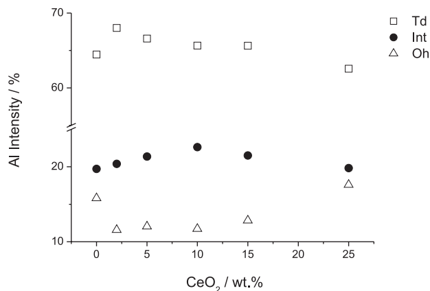
Figure 6. Plot of the distribution of tetrahedral (Td), octahedral (Oh) and intermediate (Int) aluminum sites of the Ce-USY catalysts (all calcined at 550 °C for 8 h) as a function of cerium loading.
