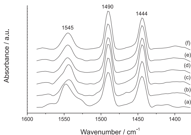
Figure 8. FTIR spectra of HUSY and Ce-USY (calcined at 550 °C for 8 h) after pyridine adsorption and thermal desorption at 150 °C: HUSY (a) and Ce-USY catalysts containing 2 (b), 5 (c), 10 (d), 15 (e) and 25% wt. of CeO 2 (f).
