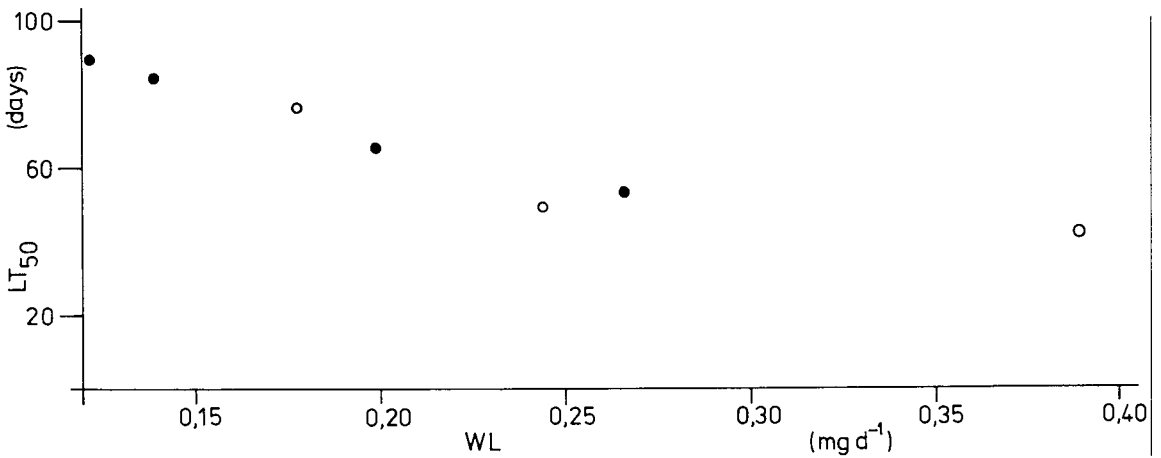
Fig. 2 – The relationship between mortality rate (LT 50) of D. maximus and the mean rate of weight loss per insect in each group (WL). Two data points were not included: for 100% RH and 34°C (see text). Temperature controlled (o), humidity controlled (●).
