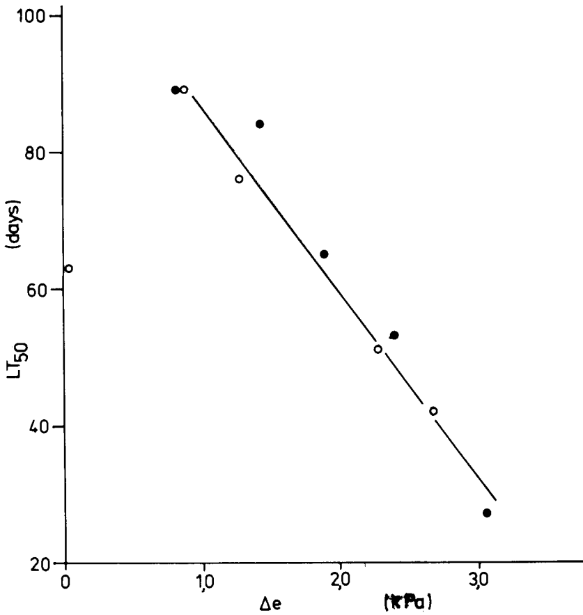
Fig. 1 – The relationship between mortality rate (LT 50) of D. maximus and the vapour pressure deficit (VPD). The linear regression line is shown. Temperature controlled (o), humidity controlled (●).
